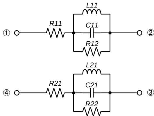
Equivalent Circuit 等価回路
