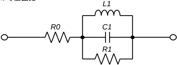
Equivalent Circuit 等価回路
