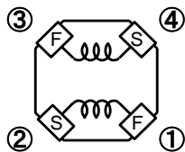
Bottom View (SQR-C series)
