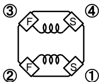
Bottom View (SQR-CA series) ※
